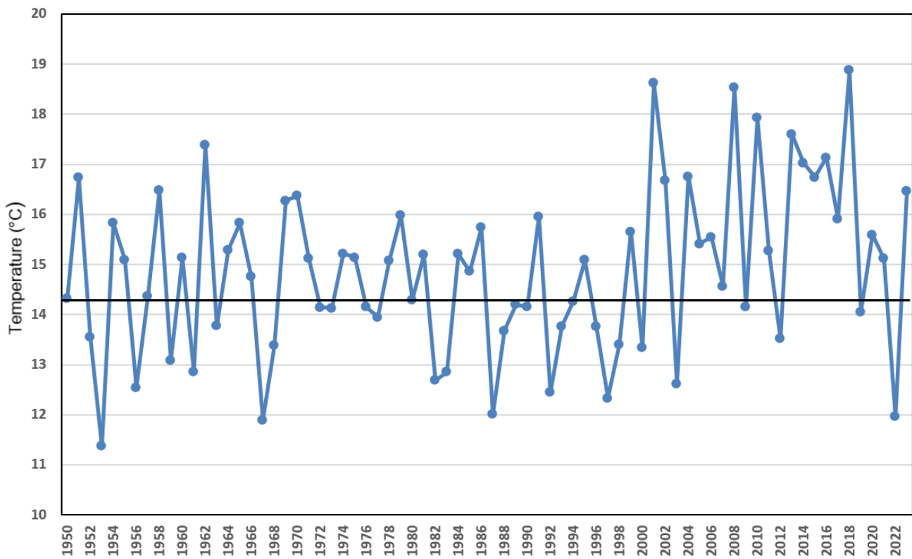
Figure 5: The average temperature in Israel* in January 1950-2023
